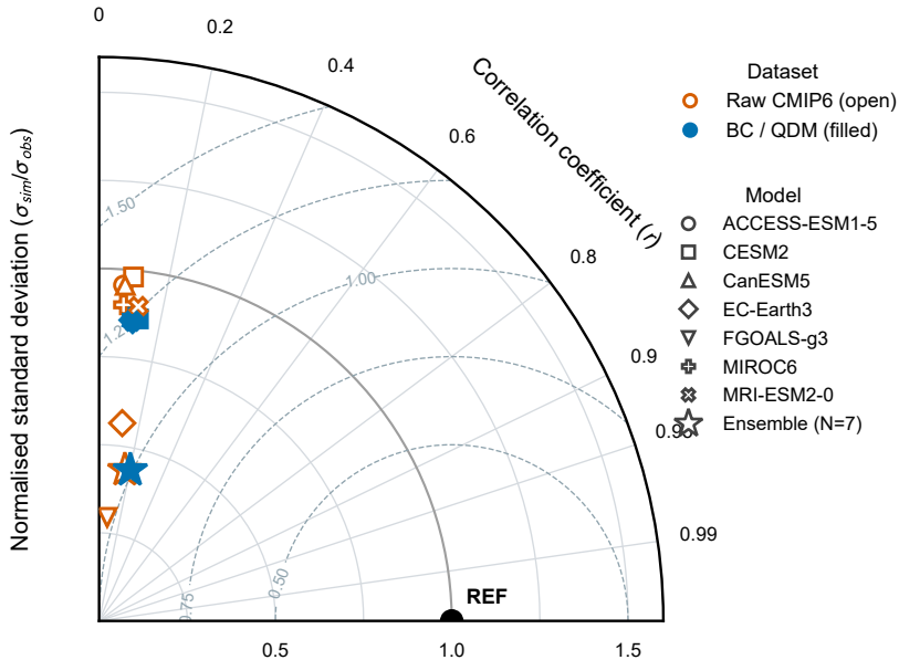
(a) Taylor diagram — daily precipitation (station-averaged, normalised)
